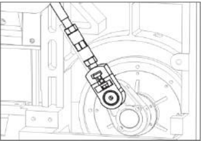
刀臂拉杆设计为内置式保险杆结构：避免由于误动作或超载对机、器产生的破坏性损坏。 Inside style asfety rod of knife holder: to avoid damage of machine caused by incorrect operation or over-loading cutting
