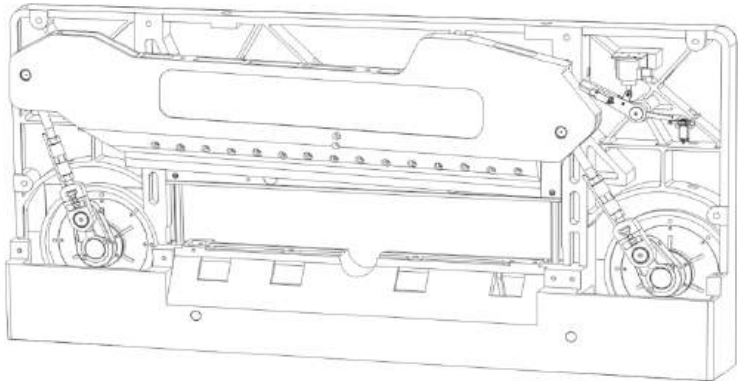
刀臂拉杆设计为内置式保险杆结构：避免由于误动作或超载对机、器产生的破坏性损坏。 Inside style asfety rod of knife holder: to avoid damage of machine caused by incorrect operation or over-loading cutting
