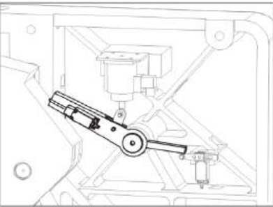
内置式电子刀锁：为切刀循环而设计的机械安全装置，避免产生滑刀的危险动作。 Knife locking latch: safety device for cutting circles to avoid dangerous of cutting sliding.
